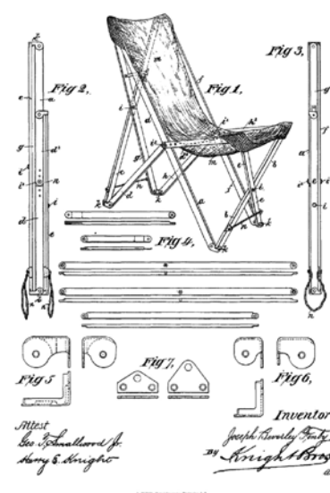
(No Model.) J. B. FENBY. FOLDING CHAIR. No. 244,216. Patented July 12, 1881.
